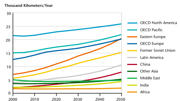
Figure 8. Projected growth in per capita transport activity
